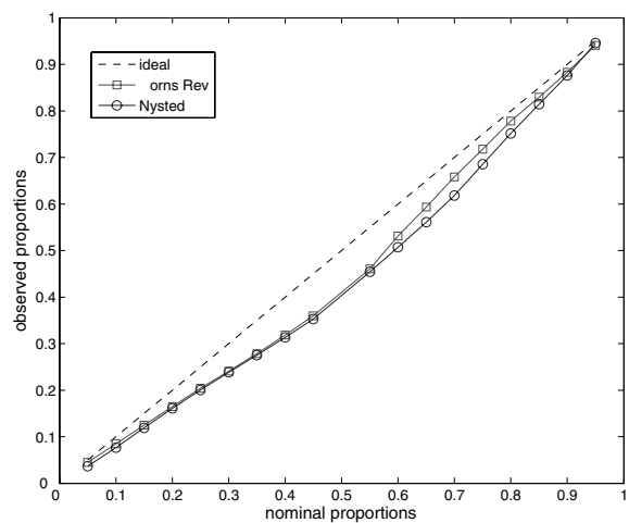
Fig. 4. Reliability evaluation of quantile forecasts obtained from the Markov-switching autoregressive models for both Horns Rev and Nysted. Such reliability diagram compare nominal and observed quantile proportions.
