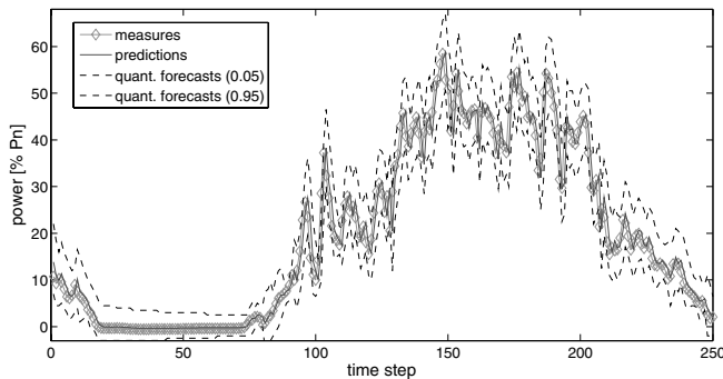
Fig. 5. Time-series of normalized power generation at Horns Rev (both measures and one-step ahead predictions) over an arbitrarily chosen episode, accompanied with prediction intervals with a nominal coverage of 90%.
