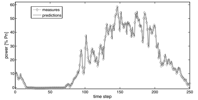
Fig. 1. Time-series of normalized power generation at Horns Rev (both measures and one-step ahead predictions) over an arbitrarily chosen episode.
