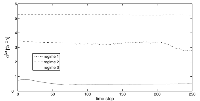
Fig. 3. Evolution of the standard deviation of conditional densities in the various regimes for the same episode.
