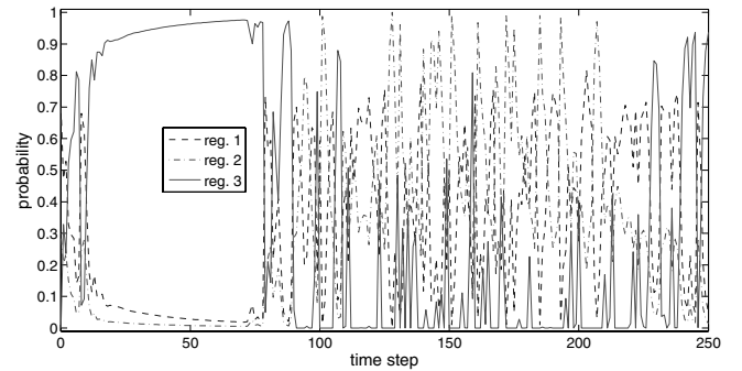
Fig. 2. Evolution of filtered probabilities given by the Markov-switching model over the same period.
