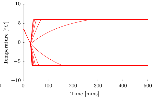
(f) Temperature, P_0 = 13 \text{ kW}
