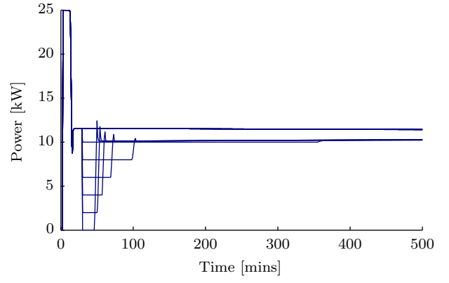
(b) Power Consumption, P_0 = 25 \text{ kW}
