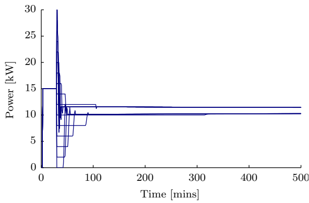
(e) Power Consumption, P_0 = 15 \text{ kW}
