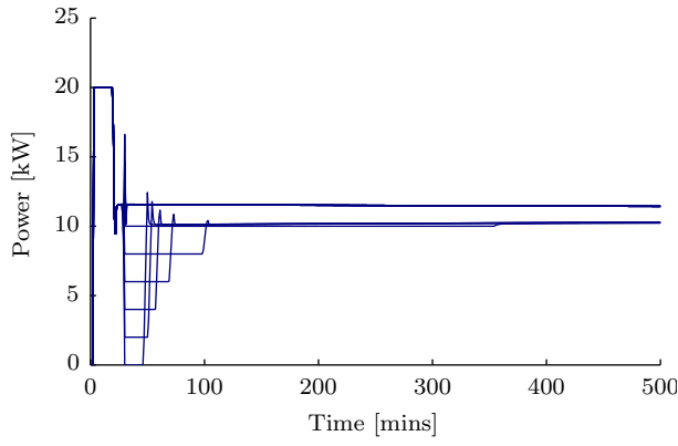
(c) Power Consumption, P_0 = 20 \text{ kW}
