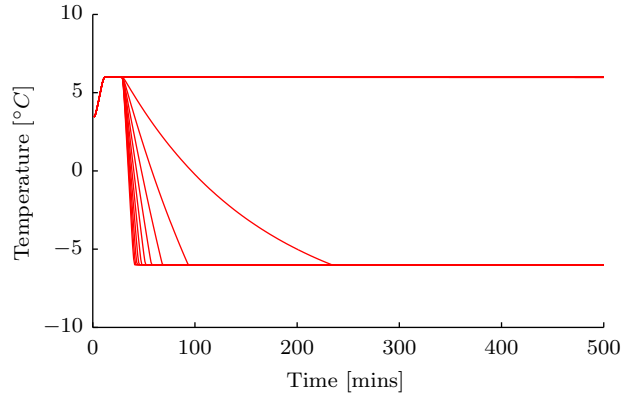
(j) Temperature, P_0 = 5 \text{ kW}
