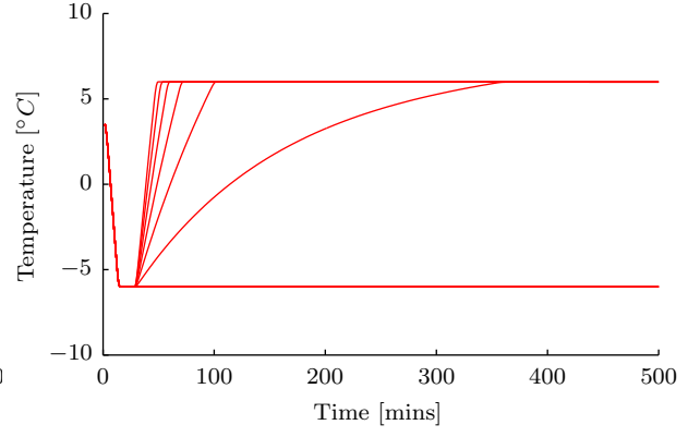
(b) Temperature, P_0 = 25 \text{ kW}
