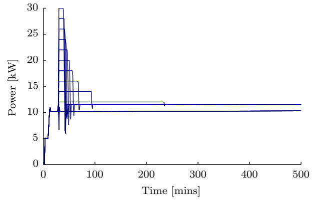
(j) Power Consumption, P_0 = 5 \text{ kW}
