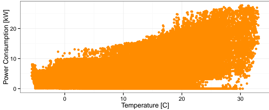
Figure 7: Relationship between Power Consumption and Outdoor Temperature
