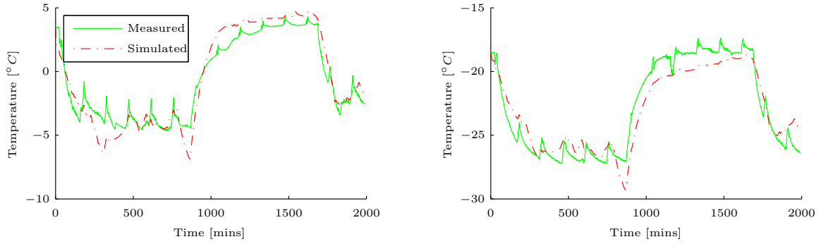
(a) Model Simulation Performance, MT Unit
