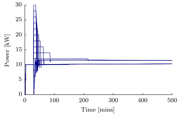
(h) Power Consumption, P_0 = 10 \text{ kW}
