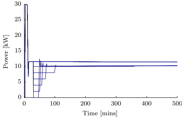
(a) Power Consumption, P_0 = 30 \text{ kW}
