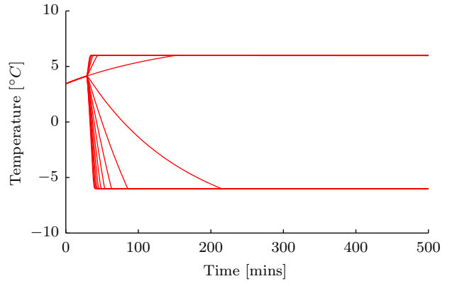
(h) Temperature, P_0 = 10 \text{ kW}
