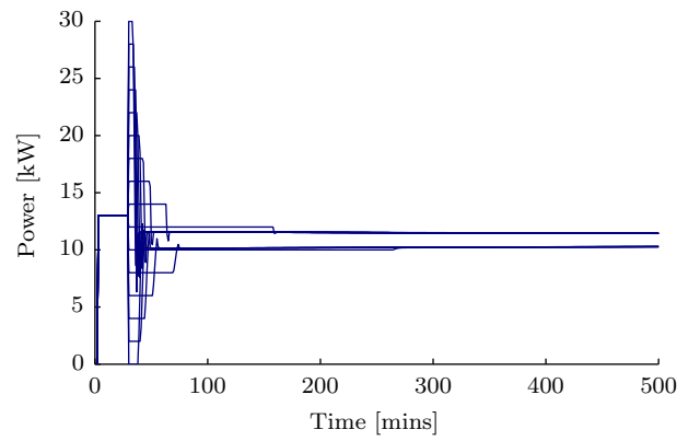
(f) Power Consumption, P_0 = 13 \text{ kW}
