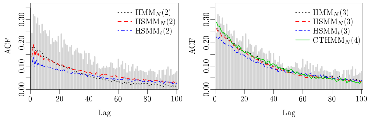
Figure B2. The empirical autocorrelation function of the squared outlier-corrected FTSE 100 log-returns at lag 1–100 together with autocorrelation functions of the squared outlier-corrected simulated log-returns for the fitted models.
