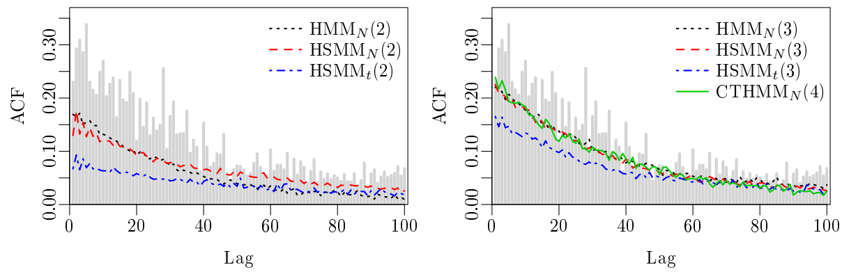
Figure B1. The empirical autocorrelation function of the squared FTSE 100 log-returns at lag 1–100 together with simulated autocorrelation functions for the fitted models.
